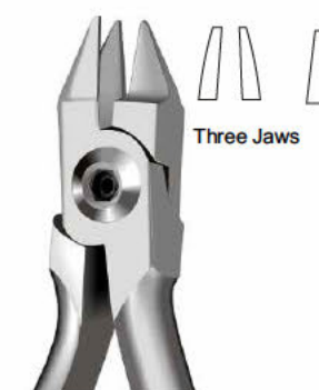
Aderer 12-4812 11.5 cm/ 4 1/2" Three Jaw Thin Plier, For wires up to .028" ( 0.71 mm ).
